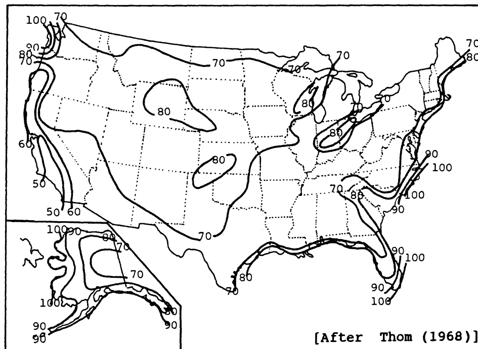
Figure 22-2 Fastest-Mile Wind Speeds: 25-year Return Period
