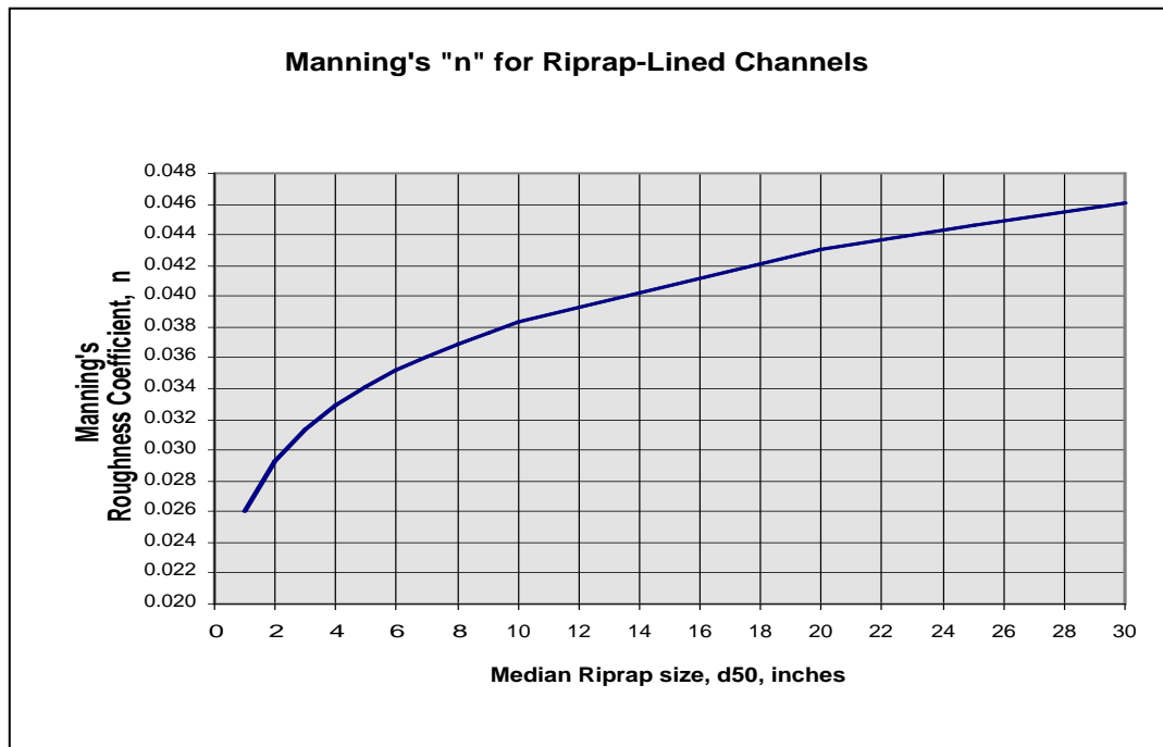
Curve 22-1
