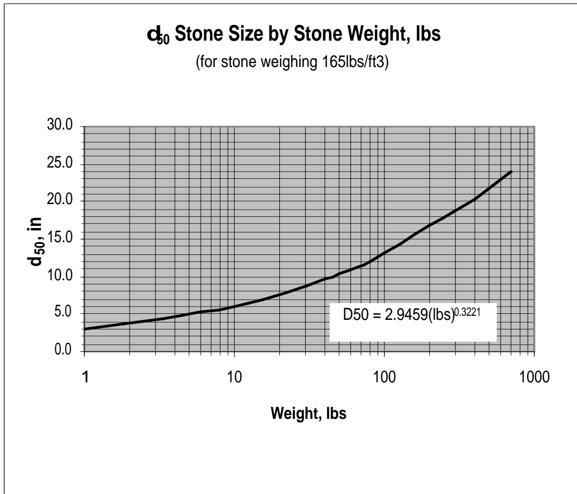
Curve 22-7
