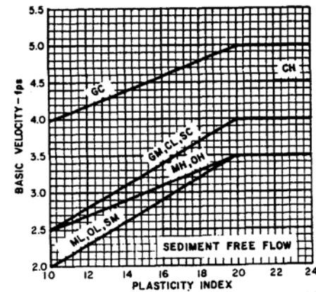
BASIC VELOCITIES FOR COHERENT EARTH MATERIALS ( v_b )
