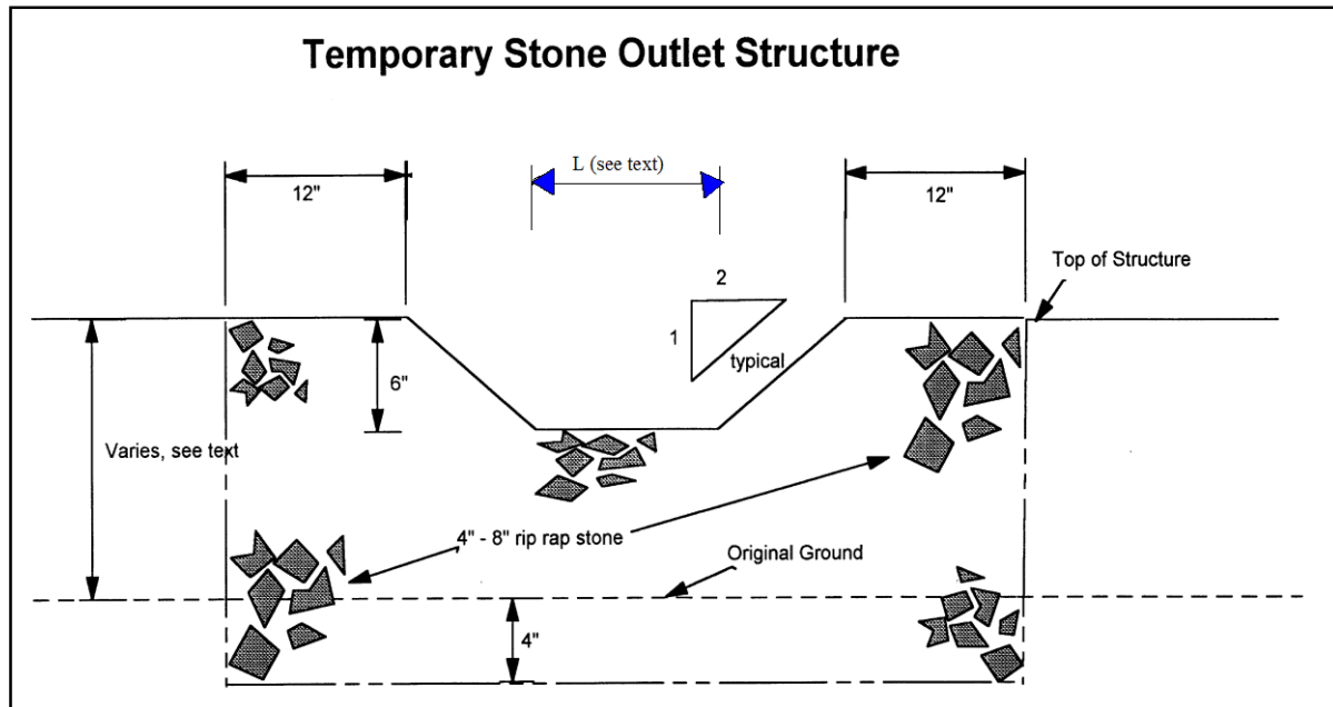
Figures 15-1 &amp; 15-2: Outlet Structure Cross Section and Profile
