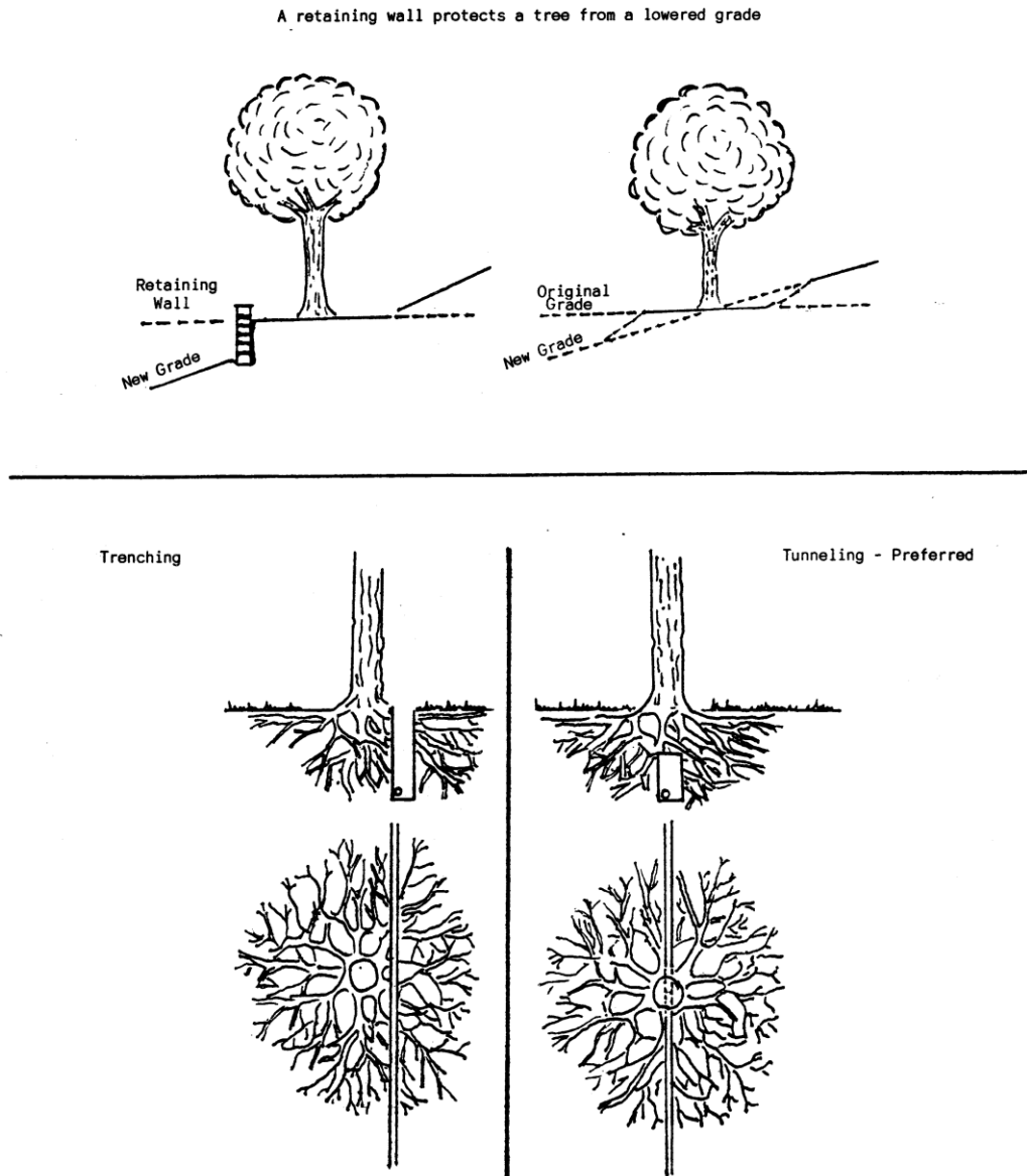
Figure 9-5: Tree Protection in Cut Areas
